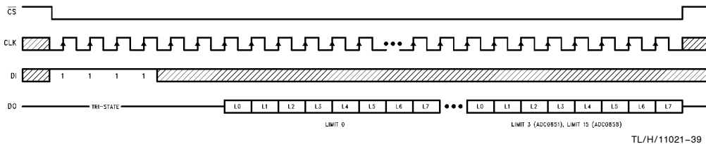
FIGURE 6. Timing Diagram for Read All Limits ADC0851/ADC0858
